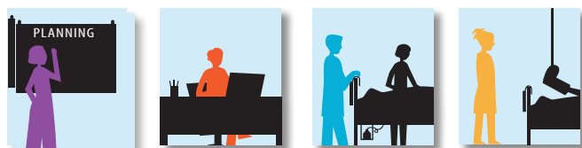
cellule formation
